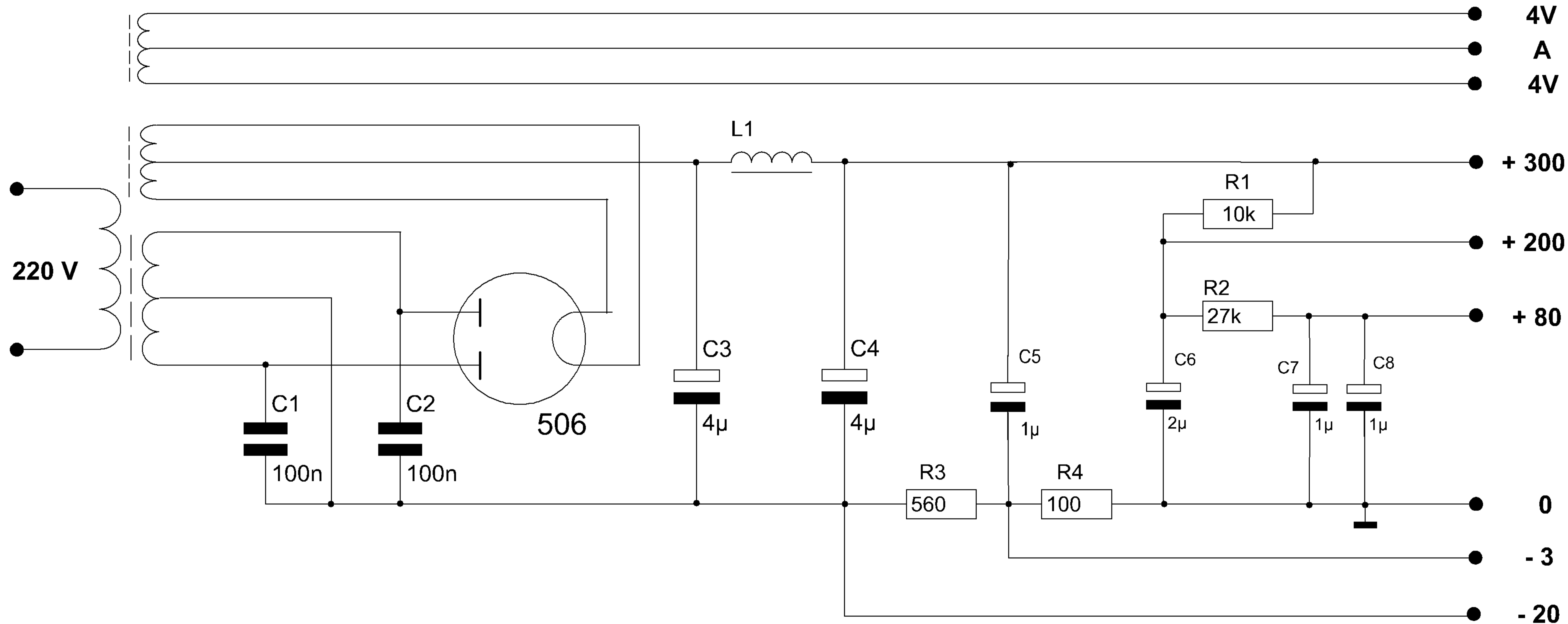
Power supply KRO PAN Europa (type VI)
